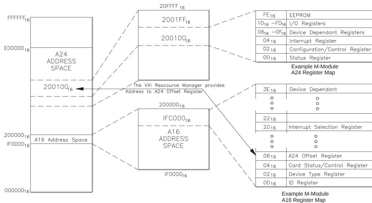
Figure 3-4. Register Mapping in A16 and A24 Address Space
