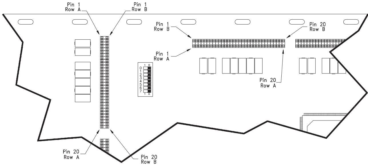
Figure 1-3. Control Interface Connector Pin Numbering
